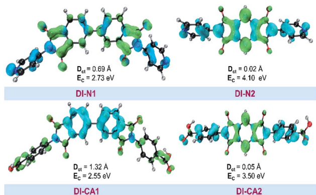
Fig. 5 Real space representation of hole and electron distributions for the studied dyes. Blue (green) regions denote the hole (electron) distributions. D_{CT} and E_C represent CT distance and exciton binding energy, respectively.
