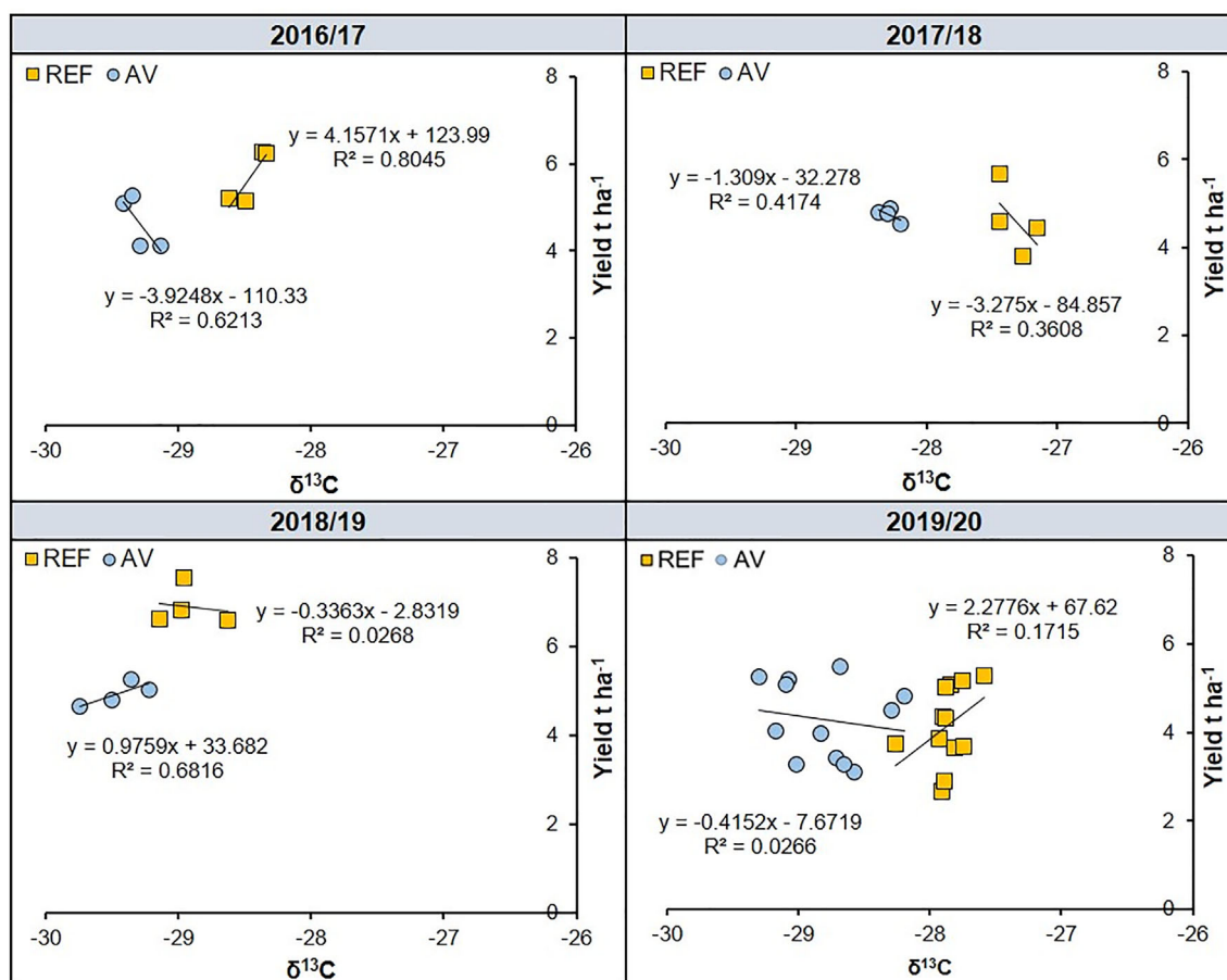
FIGURE 3 Relationship between winter wheat yield (grain, \text{t ha}^{-1} ) and \delta^{13}\text{C} (‰). Crops were harvested in four seasons (2016/17, 2017/18, 2018/19, 2019/20) either in an agrivoltaic system (AV) or on an unshaded reference site (REF) in 20 meters distance.
