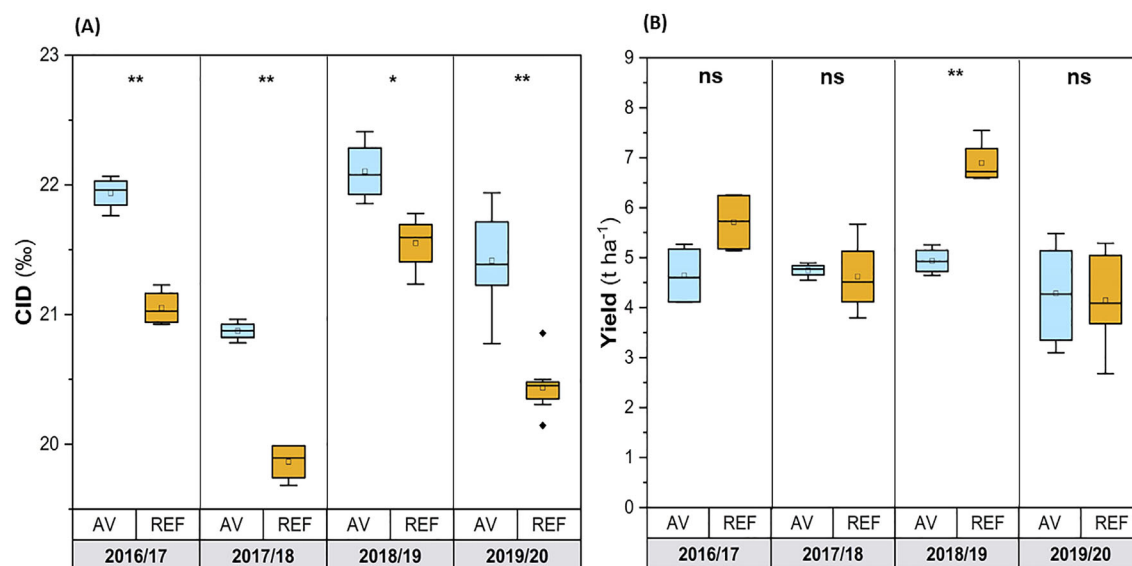
FIGURE 2 Effects of an agrivoltaic system on drought mitigation and yield: (A) Carbon-13 isotope discrimination (CID, ‰) in winter wheat grains and (B) grain yield ( \text{t ha}^{-1} ) of winter wheat cultivated in an agrivoltaic system (AV) and on an adjacent unshaded reference site (REF) between 2016–2020 at Herdwangen-Schönach (Germany). *, ** Significant differences at 0.05, 0.001 significance levels.
